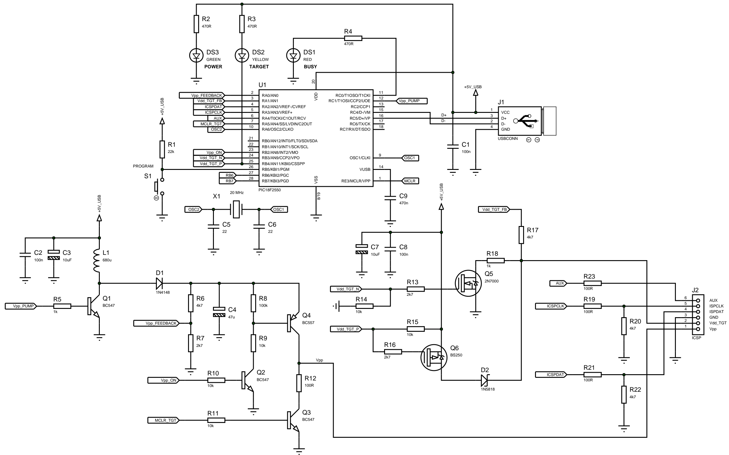
PICKit 2 Light
