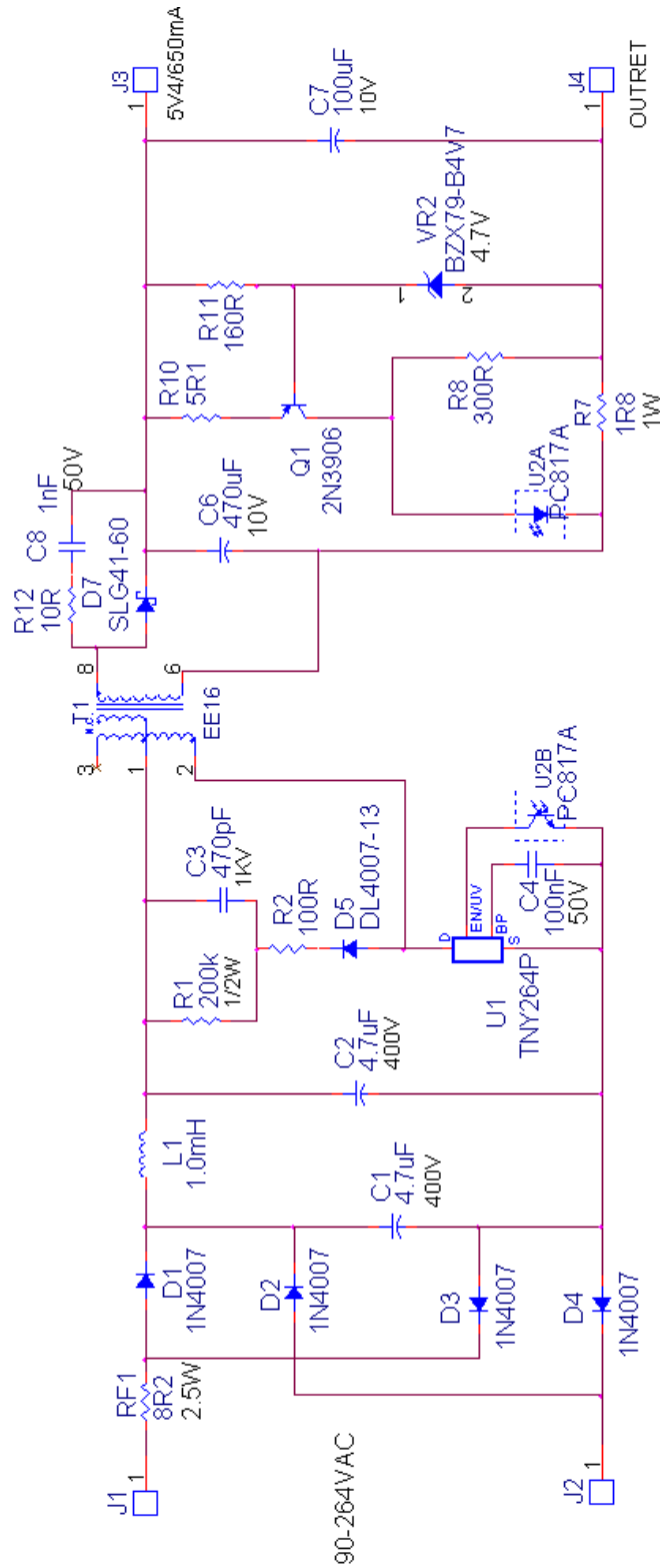
Figure 2 – Schematic.
