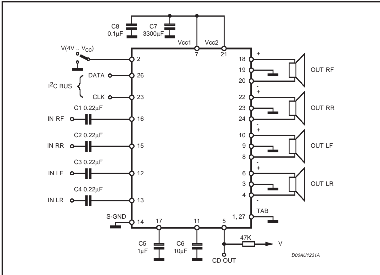
Figure 1. Application Circuit
