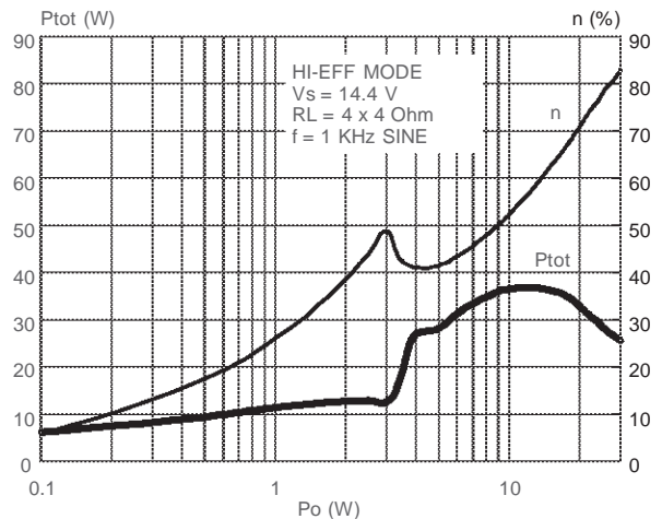
Figure 13. Power Dissipation & Efficiency vs. Output Power (4Ω, HI-EFF, SINE)
