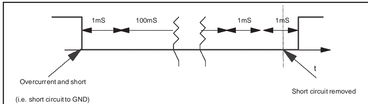
Figure 20. Restart timing with Diagnostic Enable (Permanent)
