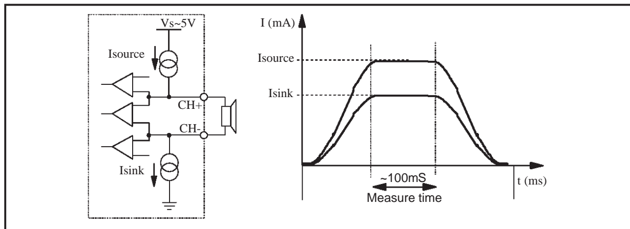
Figure 16. Turn - On diagnostic: working principle
