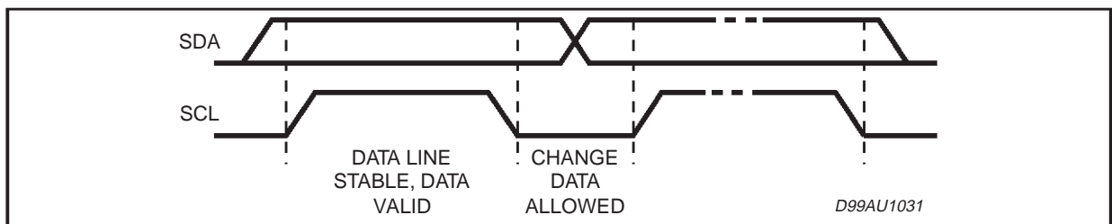
Figure 22: Data Validity on the I 2 C BUS
