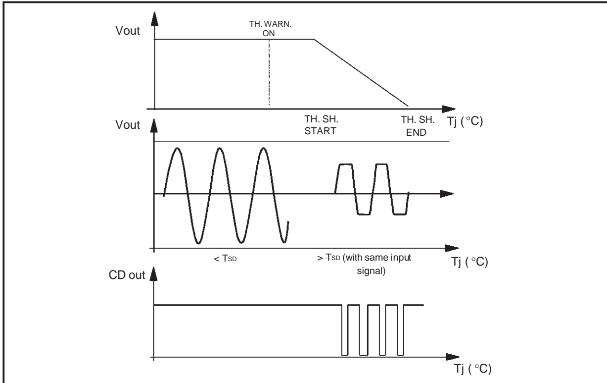
Figure 21. Thermal Foldback Diagram
