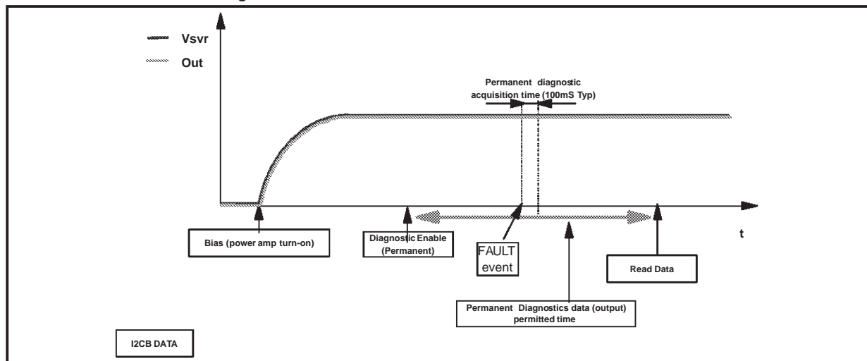
Figure 17. SVR and Output behaviour
