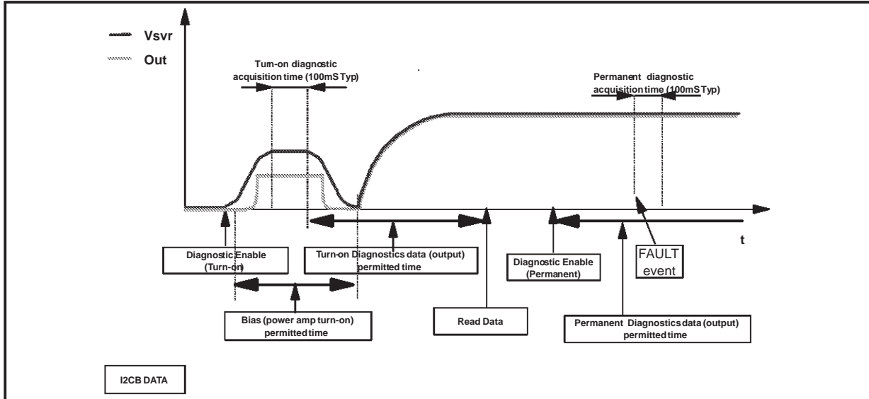
Figure 18. SVR and Output pin behaviour
