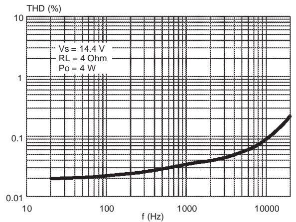
Figure 7. Distortion vs. Frequency ( 4\Omega )
