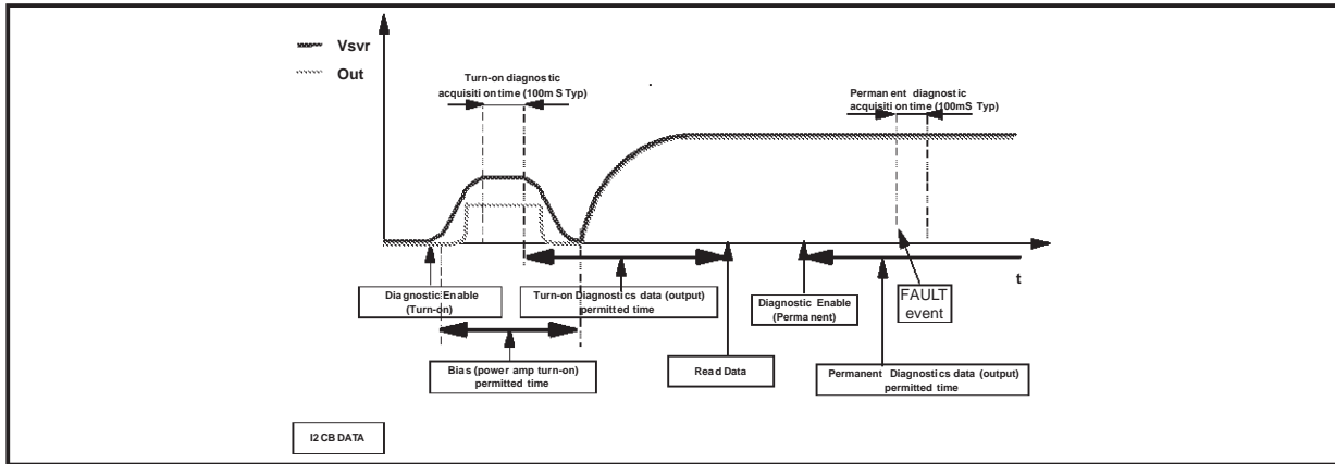
Figure 16. SVR and Output pin behaviour
