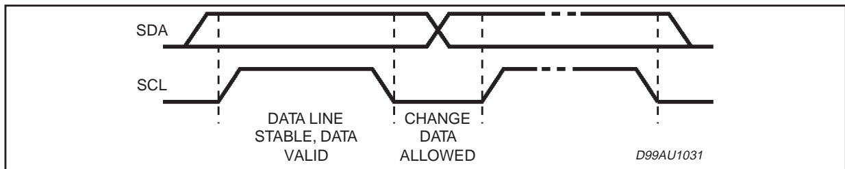
Figure 20: Timing Diagram on the I 2 C BUS
