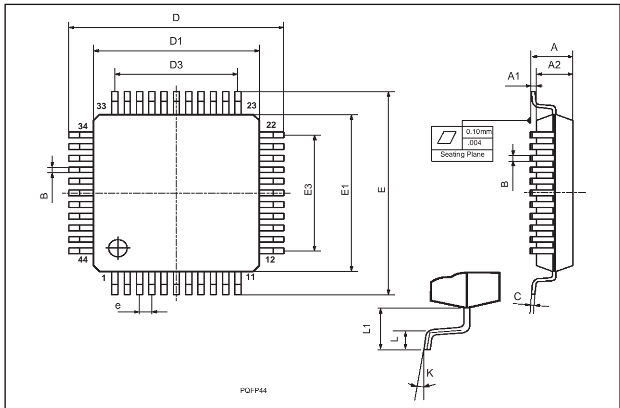
PQFP44 (10 x 10)
