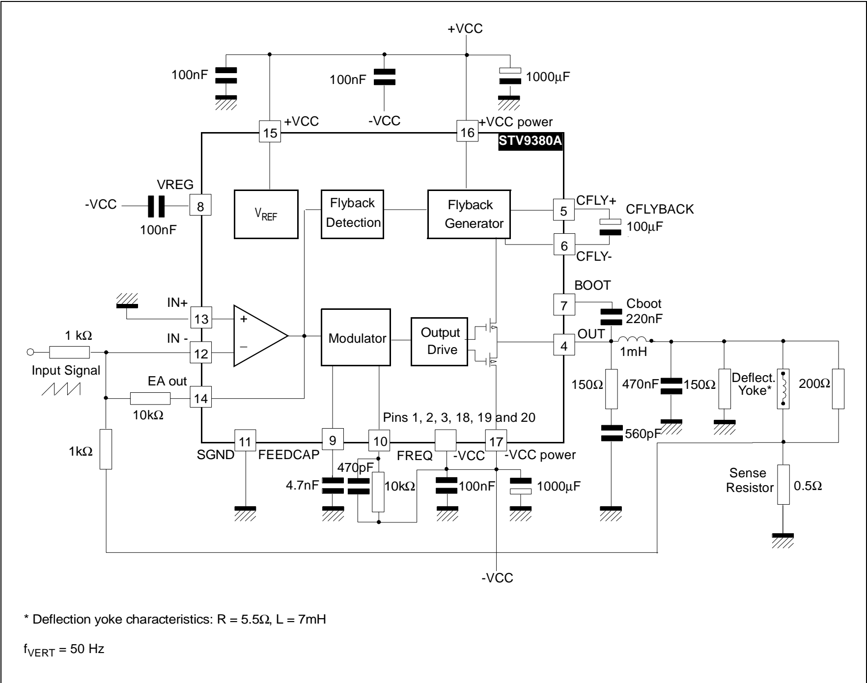
Figure 1: Test and Application Circuit Diagram
