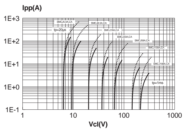
Fig. 4: Clamping voltage versus peak pulse current (Tj initial=25°C). Exponential waveform tp=20µs & tp=1ms.
