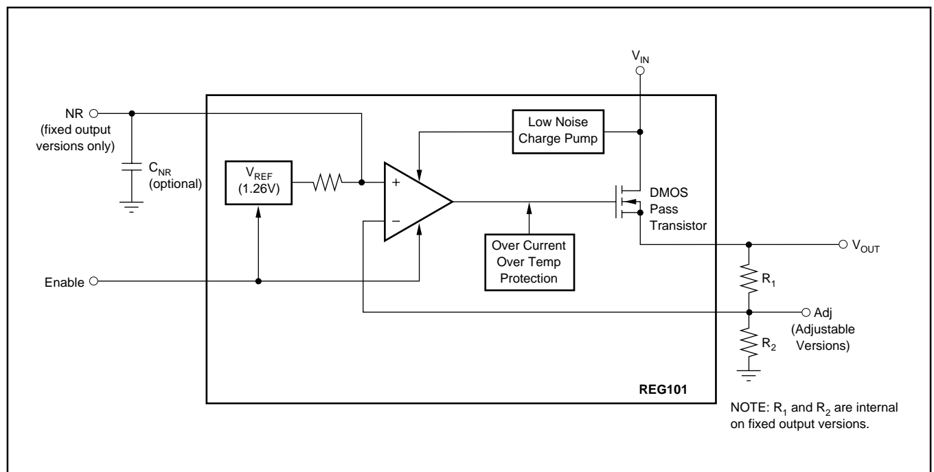
FIGURE 4. Block Diagram.
