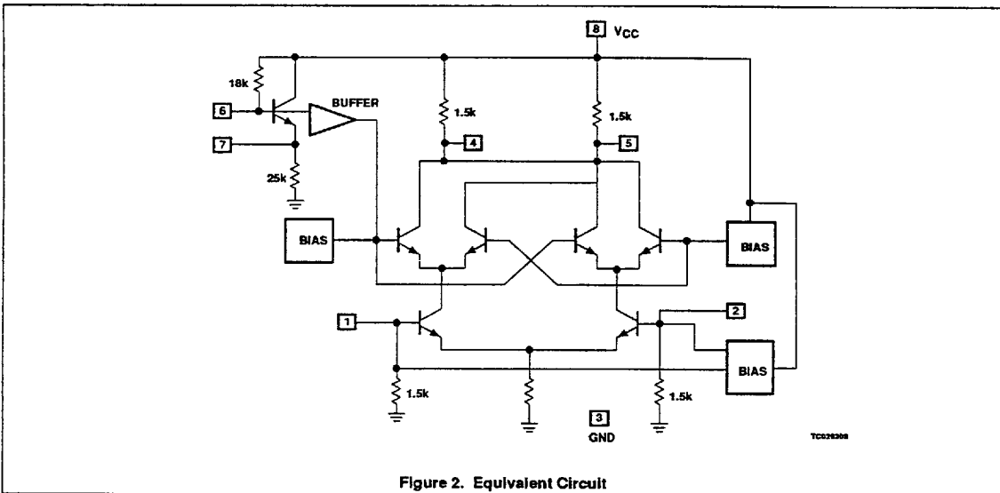
Figure 2. Equivalent Circuit
