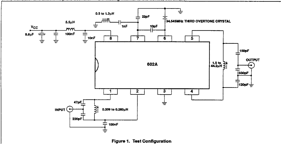
Figure 1. Test Configuration
