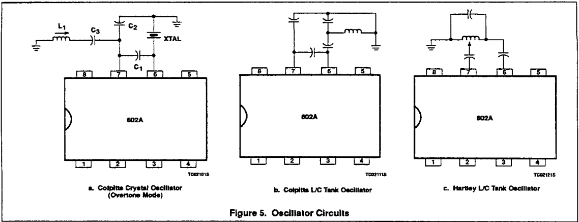
Figure 5. Oscillator Circuits
