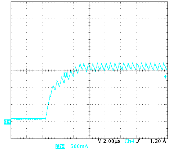
Figure 21. Short-Circuit Protection ( V_{IN} = 3.6\text{ V} , V_{OUT} = 1.2\text{ V} , I_{OUT} = CC , Temperature = 25^\circ\text{C} )
