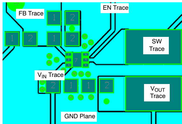
Figure 30. UDFN6 Recommended Board Layout
