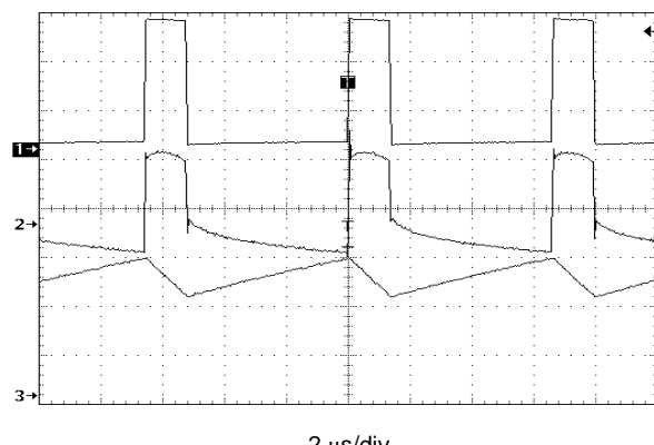
2 \mu s/div V_{OUT} = 5.0 V, V_{in} = 1.5 V, I_O = 60 mA, L = 47 \mu H, C_{OUT} = 68 \mu F 1. V_{LX} , 2.0 V/div 2. V_{OUT} , 20 mV/div, AC coupled 3. I_L , 100 mA/div
