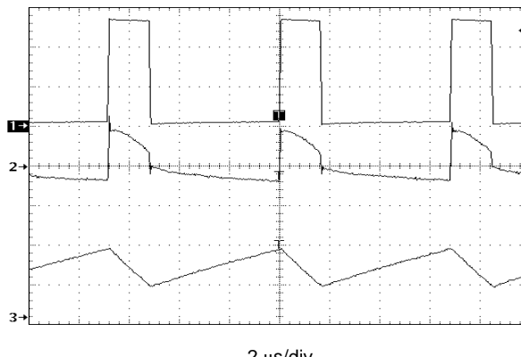
2 \mu s/div V_{OUT} = 5.0 V, V_{in} = 1.5 V, I_O = 30 mA, L = 47 \mu H, C_{OUT} = 68 \mu F 1. V_{LX} , 2.0 V/div 2. V_{OUT} , 20 mV/div, AC coupled 3. I_L , 100 mA/div
