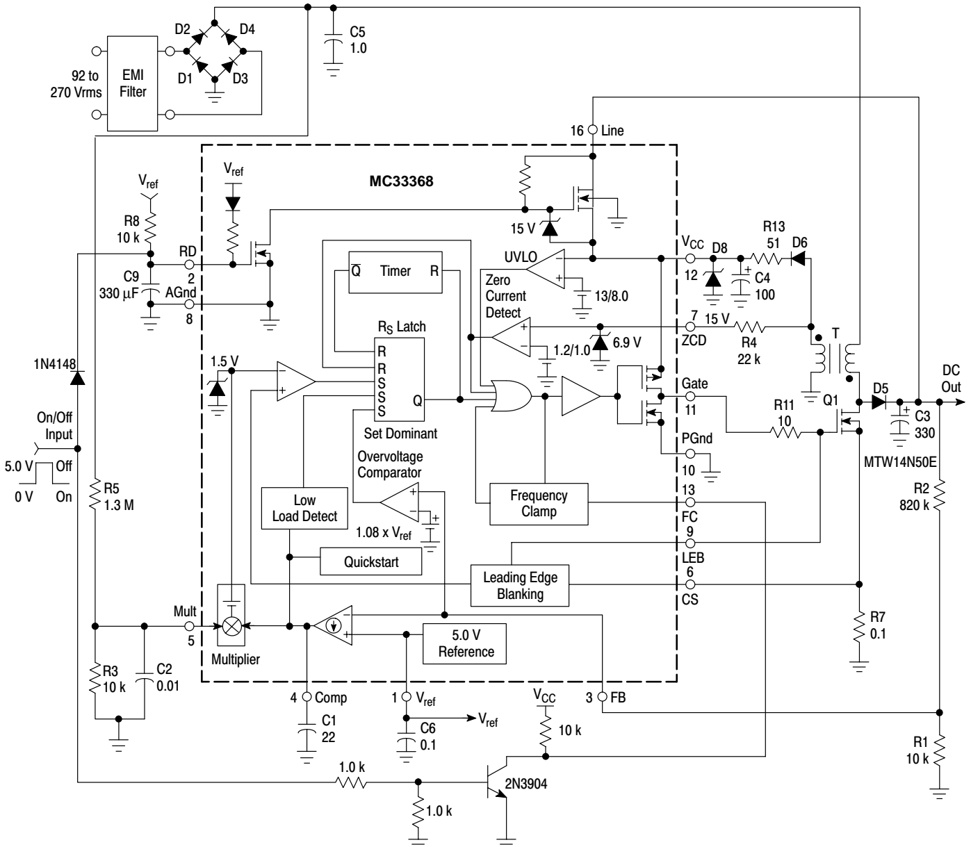
Figure 19. On/Off Control
