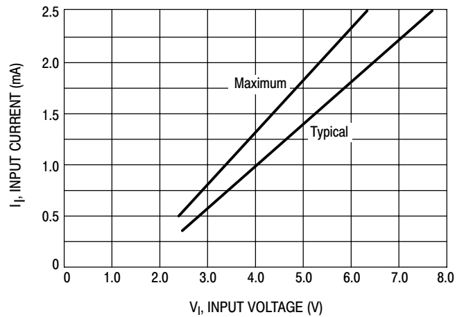
Figure 6. Input Characteristics - MC1413, B
