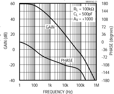
GAIN AND PHASE vs. FREQUENCY ( C_L = 500\text{pF} )
