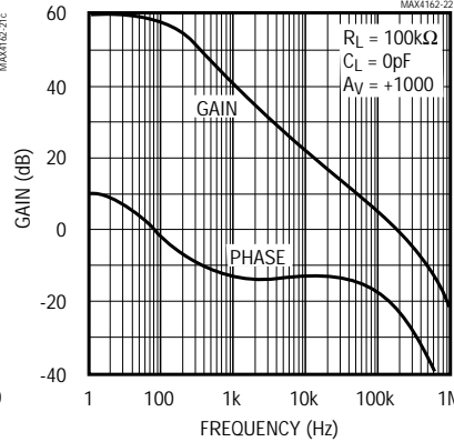
GAIN AND PHASE vs. FREQUENCY ( C_L = 0\text{pF} )
