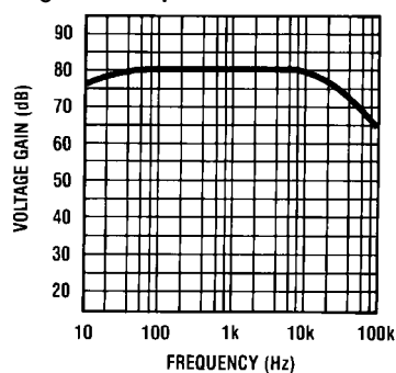
Flat Amp Voltage Gain vs Frequency V_o = 0\text{dB} , A_v = 80.0\text{dB} , f = 1\text{kHz}
