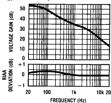
RIAA Preamp Voltage Gain RIAA Deviation vs Frequency V_{IN} = 10\text{mV} , A_v = 35.0\text{dB} , f = 1\text{kHz}
