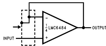
TL/H/11714-23 (c) Follower
