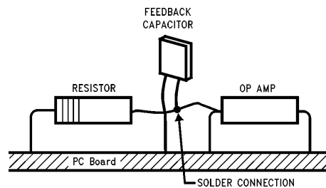
TL/H/11714-24 (Input pins are lifted out of PC board and soldered directly to components. All other pins connected to PC board.) FIGURE 11. Air Wiring
