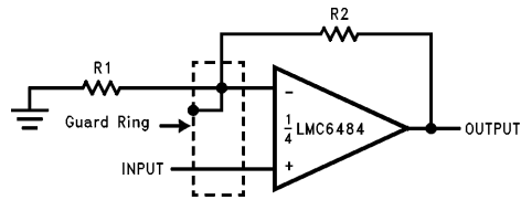
TL/H/11714-22 (b) Non-Inverting Amplifier
