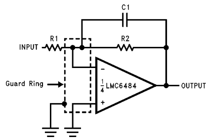
TL/H/11714-21 (a) Inverting Amplifier
