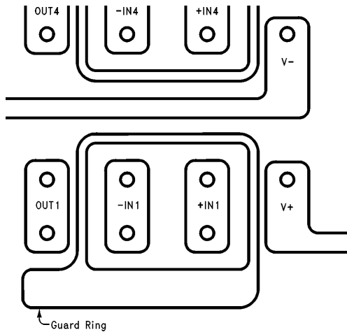
TL/H/11714-20 FIGURE 9. Example of Guard Ring in P.C. Board Layout
