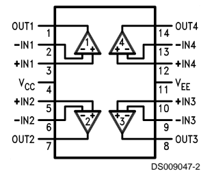
Dual-In-Line Package
