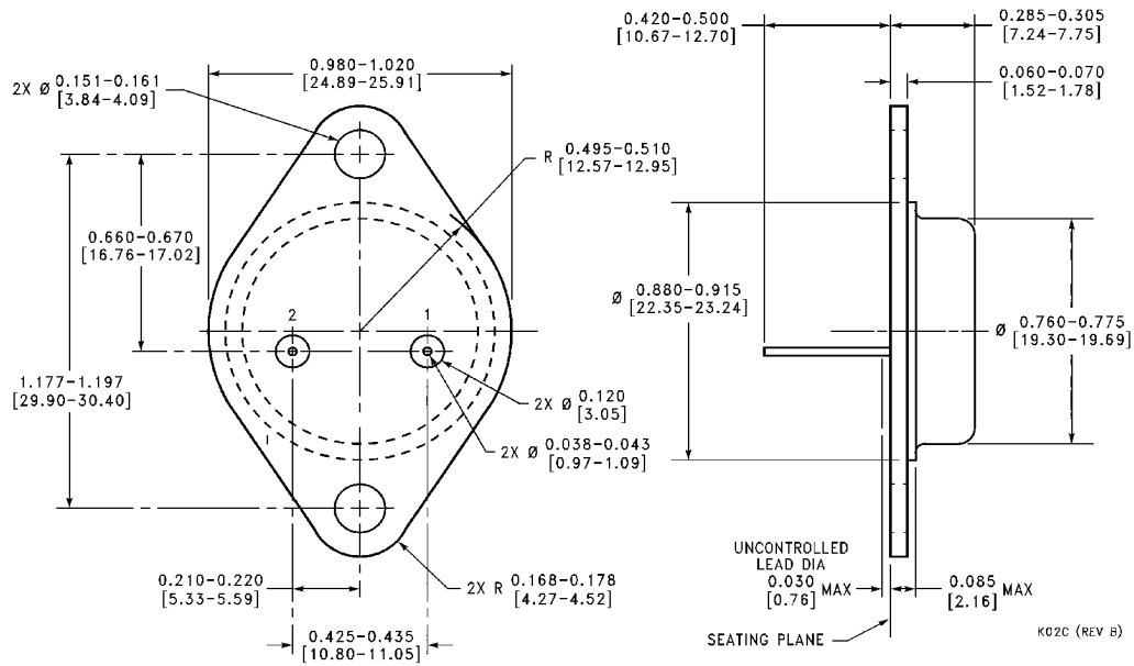
Mil-Aero Metal Can Package (K) Order Number LM137K/883 NS Package Number K02C
