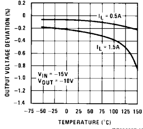
Load Regulation
