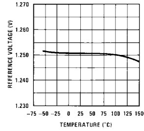
Temperature Stability
