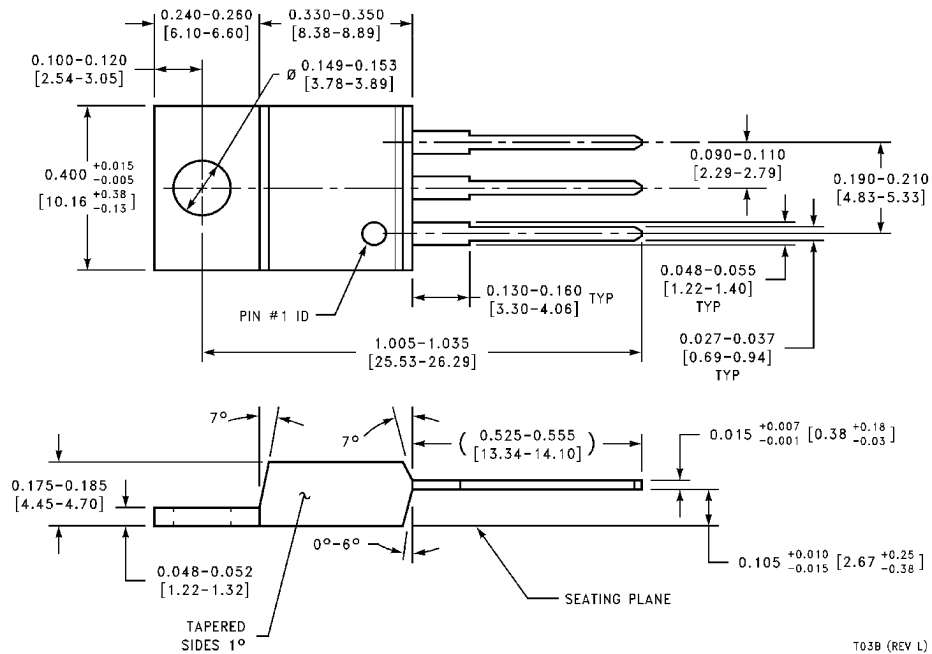
TO-220 Plastic Package (T) Order Number LM337T NS Package Number T03B
