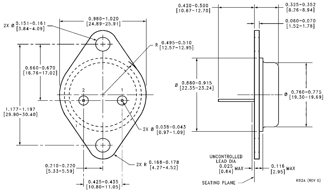
Metal Can Package (K) Order Number LM337K STEEL NS Package Number K02A
