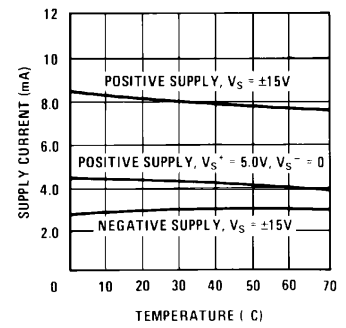
Supply Currents
