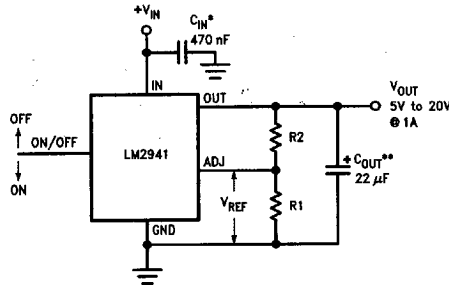
5V to 20V Adjustable Regulator
