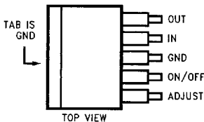
(TO-263) 5-Lead Surface-Mount Package
