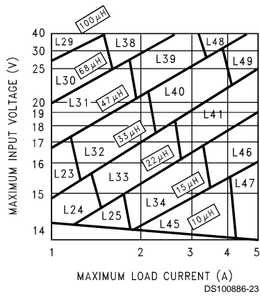
FIGURE 5. LM2678-12
