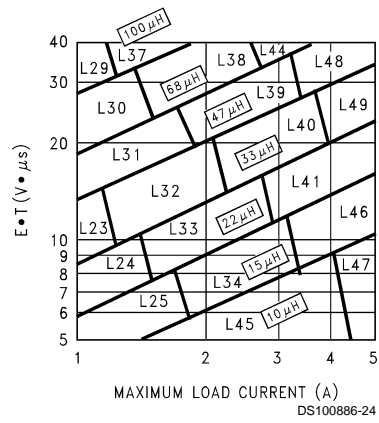
FIGURE 6. LM2678-ADJ
