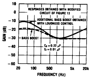
FIGURE 14. Loudness Compensated Volume Characteristic
