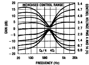
FIGURE 3. Tone Characteristic (Gain vs Frequency)
