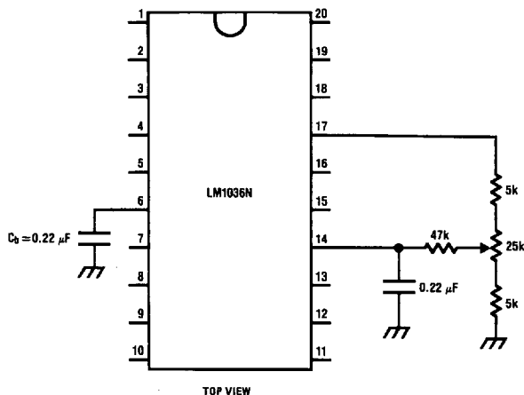
FIGURE 13. Modified Application Circuit for Additional Bass Boost with Loudness Control
