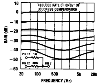
FIGURE 11. Loudness Compensated Volume Characteristic
