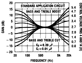
FIGURE 1. Tone Characteristic (Gain vs Frequency)
