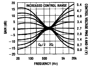
FIGURE 2. Tone Characteristic (Gain vs Frequency)
