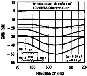
FIGURE 10. Loudness Compensated Volume Characteristic
