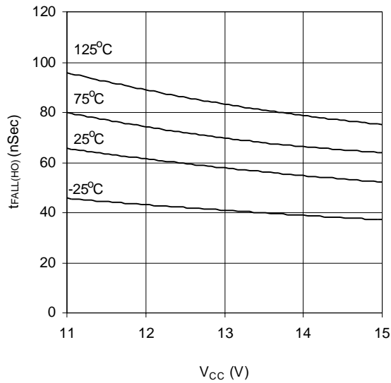
Graph 25. t_{FALL(HO)} vs V_{CC} vs Temperature (IR2156)
