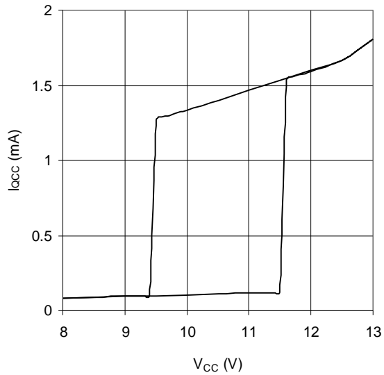
Graph 7. I_{QCC} vs V_{CC} (IR2156) UVLO Hysteresis
