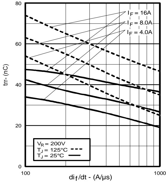
Fig. 5 - Typical Reverse Recovery vs. di_f/dt , (per Leg)
