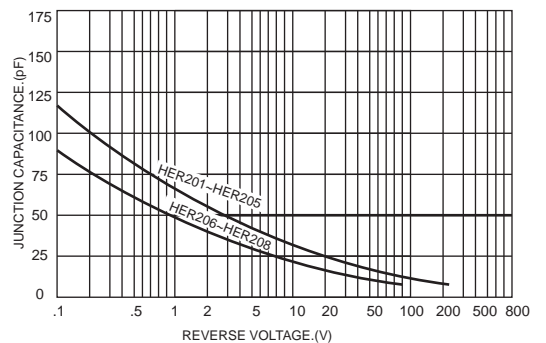
FIG.6-TYPICAL JUNCTION CHARACTERISTICS
