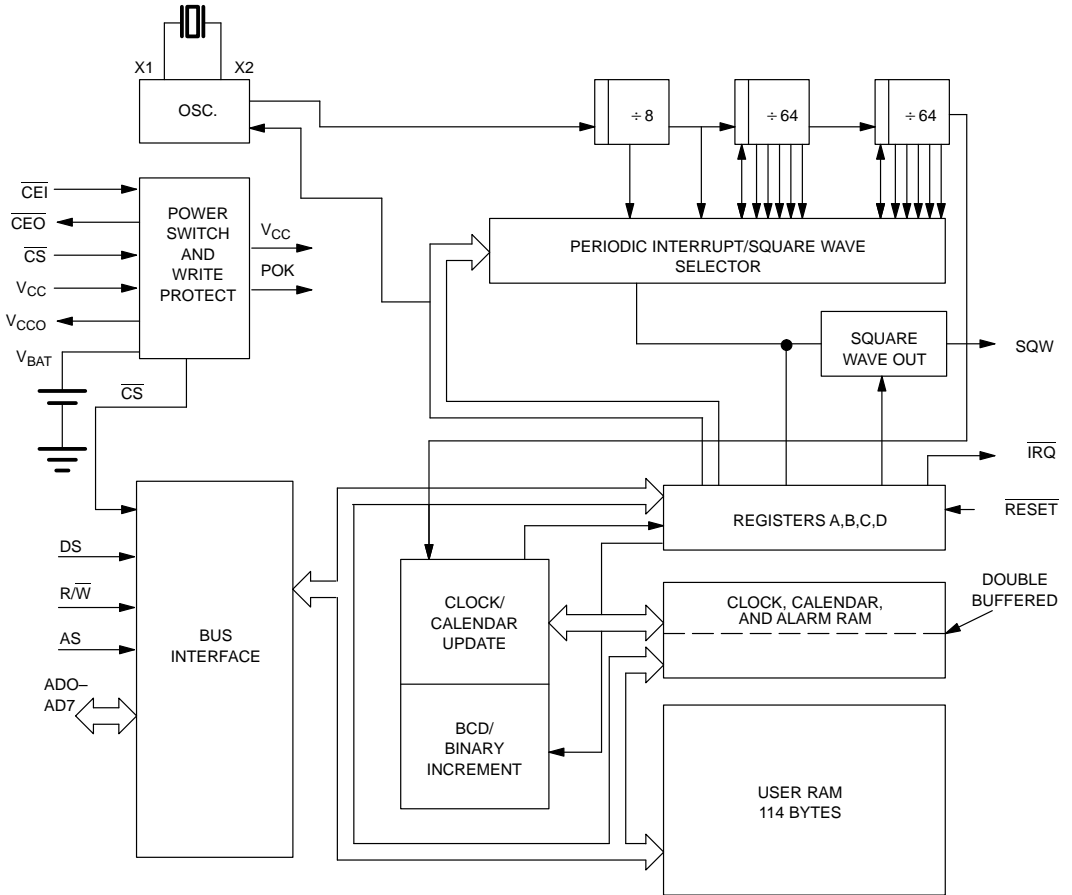
DS14285/DS14287 BLOCK DIAGRAM Figure 1
