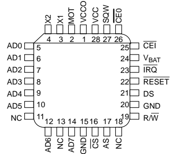
DS14285Q 28-PIN PLCC
