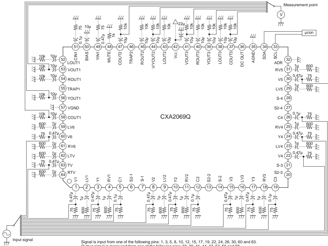
Fig. 1 Video system (gain, frequency response characteristics, input dynamic range, cross talk) measurement circuit
