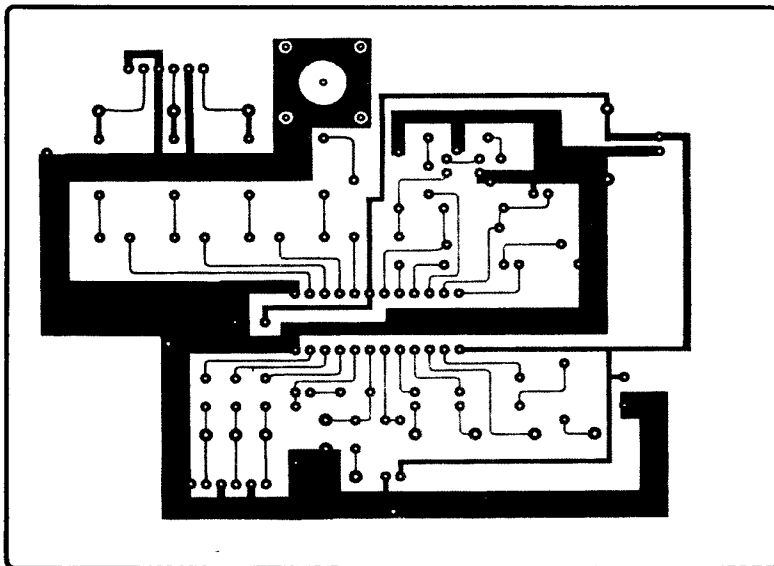
Pattern diagram (reverse side)
