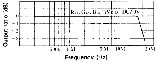
RGB output frequency characteristics
