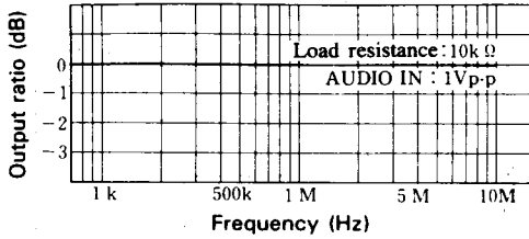
Audio buffer amplifier frequency characteristics
