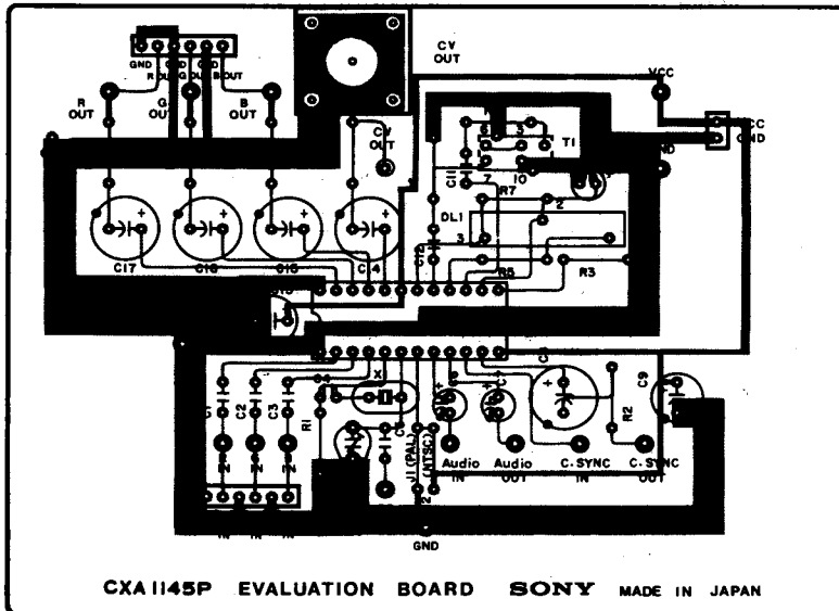
Parts arrangement diagram (parts side)
