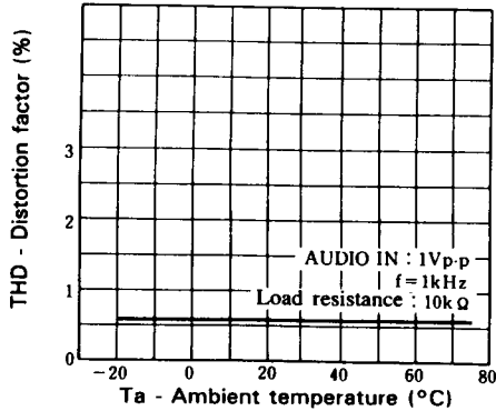
Audio buffer amplifier distortion factor temperature characteristics
