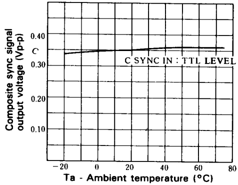
Composite sync signal output voltage temperature characteristics
