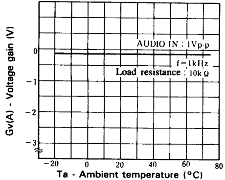
Audio buffer amplifier voltage gain temperature characteristics
