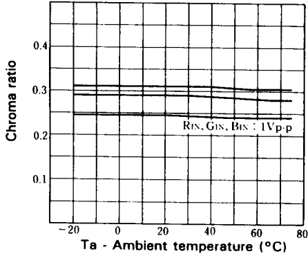
Chrome ratio temperature characteristics
