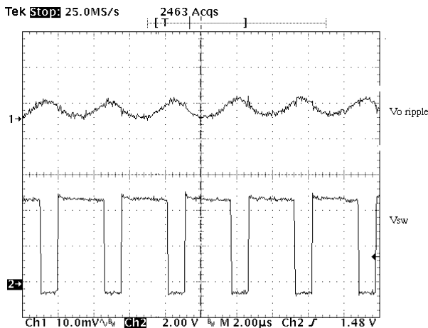
Figure 13. The Output Voltage Ripple Using Two 10 μF Ceramic Capacitors in Parallel
