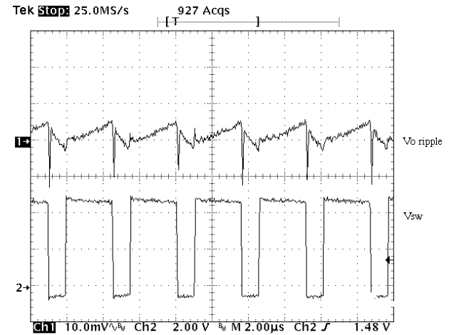
Figure 15. The Output Voltage Ripple Using One 100 μF OS-CON
