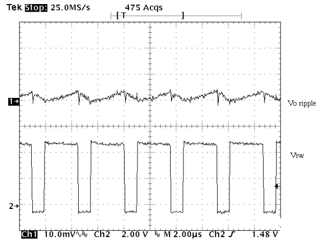
Figure 14. The Output Voltage Ripple Using One 100 μF POSCAP Capacitor
