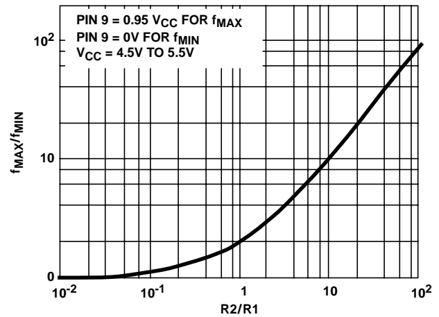
FIGURE 33. HCT4046A f_{MIN}/f_{MAX} vs R2/R1 ( V_{CC} = 4.5V \text{ TO } 5.5V )
