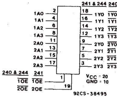
FUNCTIONAL DIAGRAM & TERMINAL ASSIGNMENT
