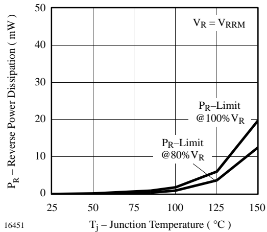
Figure 4. Max. Reverse Power Dissipation vs. Junction Temperature
