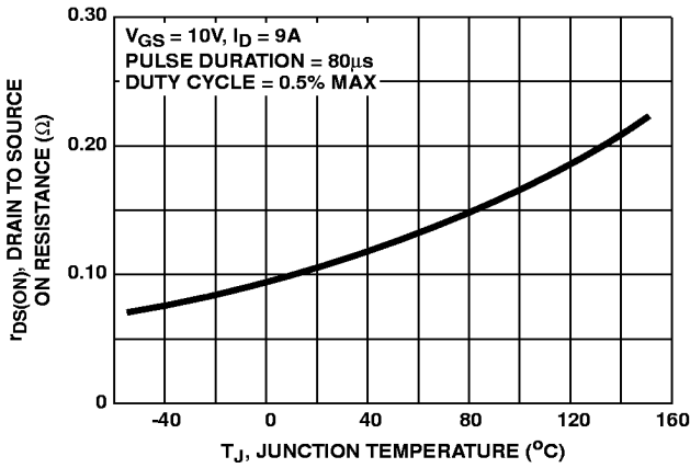
FIGURE 8. DRAIN TO SOURCE ON RESISTANCE vs JUNCTION TEMPERATURE
