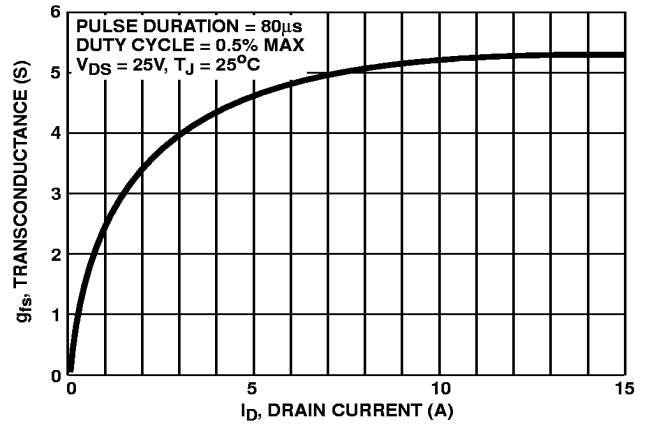
FIGURE 11. TRANSCONDUCTANCE vs DRAIN CURRENT
