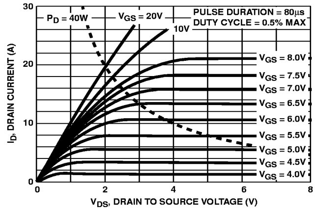
FIGURE 5. OUTPUT CHARACTERISTICS
