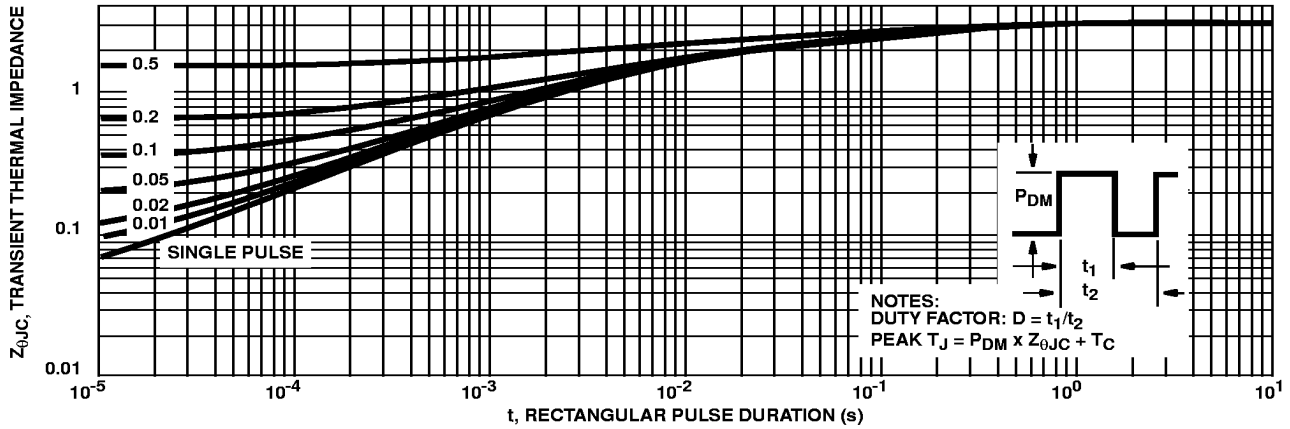
FIGURE 3. MAXIMUM TRANSIENT THERMAL IMPEDANCE
