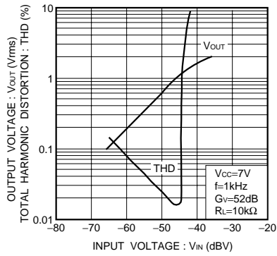
Fig.18 Input/output characteristics
