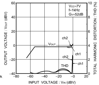
Fig.17 ALC characteristics
