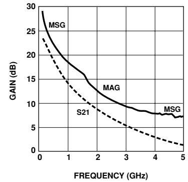
Figure 10. AT-41511 Gains vs. Frequency at V_{CE} = 2.7 V , I_C = 5 mA .
