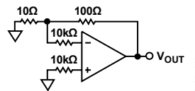
Figure 41. Current Noise Measurement Circuit
