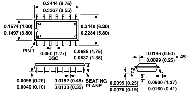
14-Lead SOIC (R Suffix)
