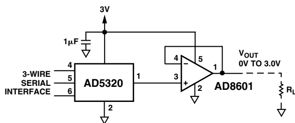
Figure 7. Using the AD8601 as a DAC Output Buffer to Drive Heavy Loads
