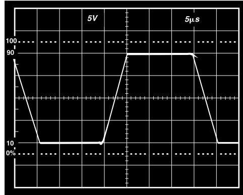
Figure 6. Large Signal Response Unity Gain Follower; V_S = \pm 15\text{ V} , R_L = 10\text{ k}\Omega
