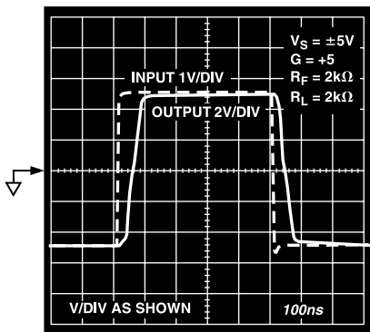
Figure 5. Overdrive Recovery
