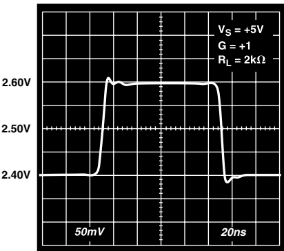
TPC 21. 200 mV Step Response; V_S = +5\text{ V} , G = +1
