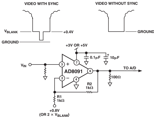
Figure 8. Sync Stripper
