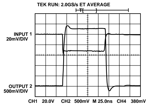
Figure 22. Pulse Response
